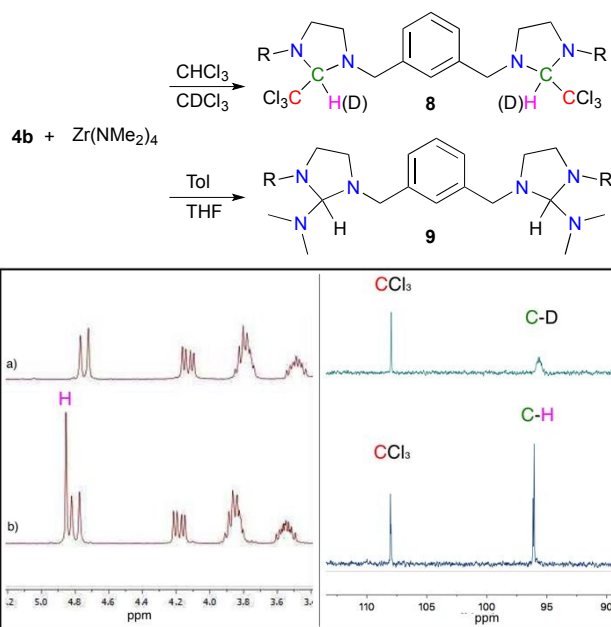
Fig. 6 Reaction leading to chloroform and dimethylamine adducts 8 and 9 , respectively (top) and an expanded view of the ^1\text{H} NMR (bottom left) and ^{13}\text{C} (bottom right) of 8-d 2 (a) and 8 (b), which show the inclusion of deuterium into the molecule.
