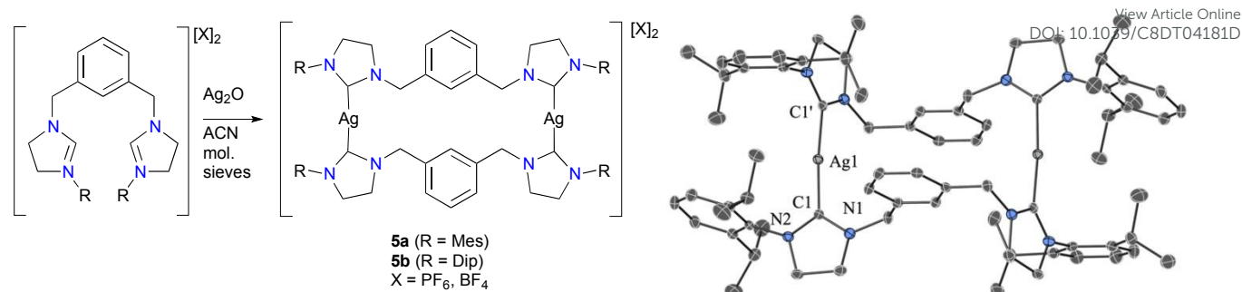
Fig. 4 Synthesis of Silver complexes 5 (left) and X-ray crystal structure of [ 5b ][PF 6 ] 2 showing the silver bridged dimer structure (right). The hydrogen atoms, PF 6 counterions, and solvent molecules (acetonitrile) have been omitted for clarity. Thermal ellipsoids at 50% probability. Bond lengths (Å) and angles (°): C1-Ag1 = 2.0971(12), C1'-Ag1 = 2.1020(12), N1-C1-C2 = 108.25(10), C1-Ag1-C1' = 174.41(4).
