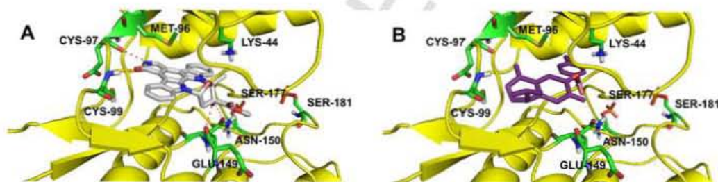
Fig. 5. Docking of staurosporine analog K252 and compound 13 at the protomer B of the human IKK \beta crystal structure (PDB ID: 4kik). (A) Staurosporine analog K252 interacts with the ATP-binding pockets through hydrogen bonds with the amino acids Cys-97, Cys-99, Glu-149 and Asn-150 (B) Compound 13 interacts with the ATP-binding pockets by Van der Waals forces ( \Delta G = -9.43 kcal/mol).
