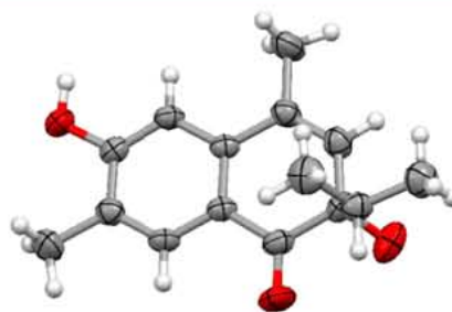
Figure 8. ORTEP drawing of the X-ray crystal structure of 7.
