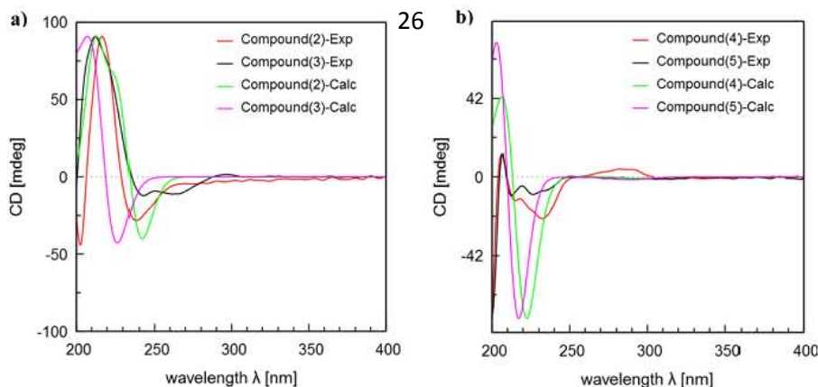
Figure 4. Calculated ECD spectra of (a) 2 (4 R ,10 S )- and 3 (4 R ,10 S )-isomers and (b) 4 (4 R )- and 5 (1 R ,4 R )-isomers and comparison with their respective experimental ECD spectra. The calculation was performed with the \pi -electron SCF-CI-DV MO method.
