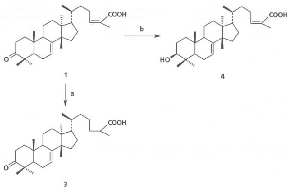
Figure 2 Reactions of masticadienonic acid ( 1 ) to produce 24,25S-dihydmasticadienonic acid ( 3 ) (55% yield), and masticadienolic acid ( 4 ) (86% yield). a, 5% Pd-C/EtOAc; b, NaBH 4 /MeOH.
